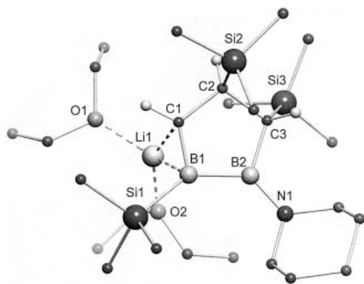
Figure 4. Structure of 7b ·Li[Et 2 O] 2 in the crystal; selected bond lengths [pm] and angles [°], the corresponding values for the second independent ion pair are provided in brackets: B1–B2 171.3(3) [170.0(4)], B1–C1 146.1(3), B2–C3 160.1(3), C1–C2 151.9(3) [152.3(3)], C2–C3 157.4(3) [156.2(3)], B1–Si1 200.9(2) [201.2(2)], B1–Li1 238.9(5) [238.3(4)], C1–Li1 239.7(5) [243.1(4)], C1–B1–B2 101.4(2) [101.8(2)], C3–B2–B1 107.2(2) [106.9(2)], C2–C1–B1 117.2(2) [116.9(2)], C2–C3–B2 105.1(2) [104.9(2)]; sum of angles (without Li1) C1 359.6 [359.2], N1 359.1 [359.3]
