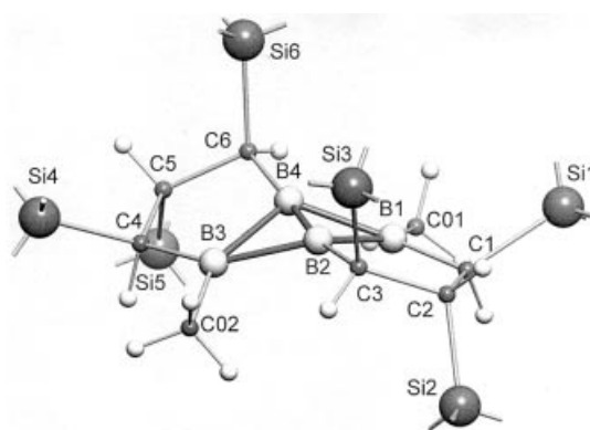
Figure 7. Structure of cis - 14 in the crystal; selected bond lengths [pm] and angles [°]: B1–B2 179.9(3), B2–B3 183.0(3), B3–B4 180.2(3), B4–B1 183.5(3), B2–B4 150.1(3), B1–C01 164.8(3), B3–C02 160.9(3), B1–C1 159.6(2), C1–C2 156.1(2), C2–C3 157.0(2), C3–B2 158.0(2); C01–B1–C1 112.0(2), C02–B3–C4 113.0(2), C3–B2–B4 169.4(2), C6–B4–B2 170.1(2), B1–B2–B4–B3 140.2(1)
