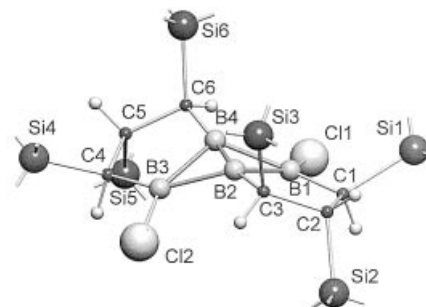
Figure 6. Structure of cis - 11 in the crystal; selected bond lengths [pm] and angles [°]: B1–B2 182.6(2), B2–B3 186.3(2), B3–B4 182.2(2), B4–B1 186.0(2), B2–B4 150.2(2), B1–Cl1 179.8(2), B3–Cl2 179.8(2), B1–C1 157.1(2), C1–C2 155.6(2), C2–C3 157.1(2), C3–B2 156.4(2); Cl1–B1–C1 112.1(1), Cl2–B3–C4 112.0(1), C3–B2–B4 169.4(1), C6–B4–B2 170.1(1), B1–B2–B4–B3 135.2(1)
