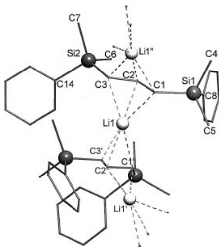
Figure 1. Section of the spiral chain with Li1 in the crystal structure of 5b ·Li; selected bond lengths [pm] and angles [°], the corresponding values for the second spiral chain with Li2 are provided in brackets (same e.s.d.s): C1–C2 140.6(4) [140.2], C2–C3 140.0(4) [139.9], C1–Li1 231.4(6) [233.9], C2–Li1 215.8(6) [215.6], C3–Li1 231.8(6) [228.7], C1'–Li1 228.8(6) [229.7], C2'–Li1 219.3(6) [216.2], C3'–Li1 235.3(6) [229.7], C1–C2–C3 129.9(3) [128.9], C2–C1–Si1 123.2(2) [124.4], C2–C3–Si2 123.8(2) [123.5], Si1–C1–C2–C3 –176.1(2) [177.9]
