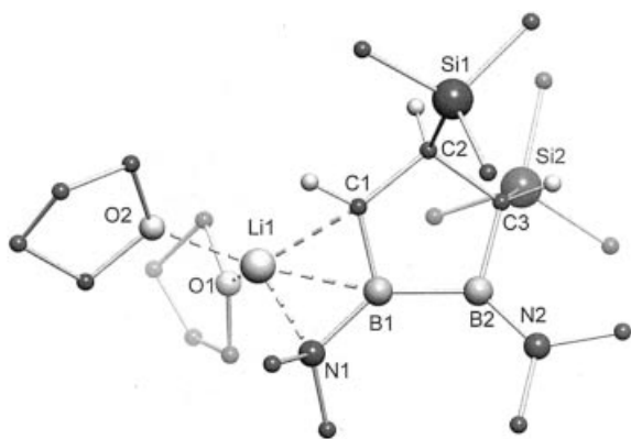
Figure 3. Structure of 7a ·Li[THF] 2 in the crystal (most H atoms have been omitted for clarity); selected bond lengths [pm] and angles [°]: B1–B2 169.1(3), B1–C1 146.6(3), B2–C3 160.8(3), C1–C2 152.4(2), C2–C3 156.8(3), N1–Li1 203.3(4), B1–Li1 230.2(4), C1–Li1 223.6(4); C1–B1–B2 103.1(2), C3–B2–B1 105.1(2), C2–C1–B1 115.4(2), C2–C3–B2 104.9(2), sum of angles (without Li1) C1 359.6, N1 344.7, N2 359.8
