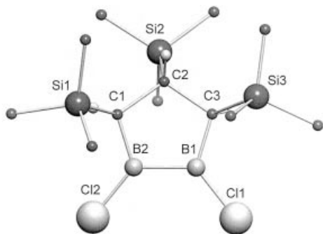
Figure 5. Structure of 1b in the crystal; selected bond lengths [pm] and angles [°]: B1–B2 169.2(4), B2–C1 150.1(4), C1–C2 156.0(3), C2–C3 157.7(3), C3–B1 151.6(3), B1–Cl1 176.0(3), B2–Cl2 175.9(3), C1–Si1 193.0(2), C2–Si2 189.9(2), C3–Si3 192.5(2); B1–B2–C1 107.2(2), B1–B2–Cl2 128.3(2), B2–B1–C3 106.4(2), B2–B1–Cl1 128.3(2), B1–C3–C2 107.4(2), C3–C2–C1 109.8(2), C2–C1–B2 107.5(2), C1–B2–B1–C3 4.5(2)
