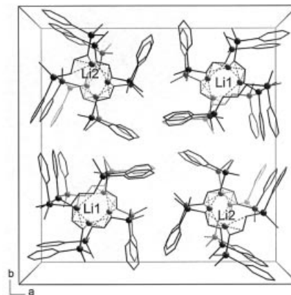
Figure 2. Perspective view along the c axis of the unit cell of 5b ·Li having alternating clockwise (Li1) and anticlockwise (Li2) spiral chains
